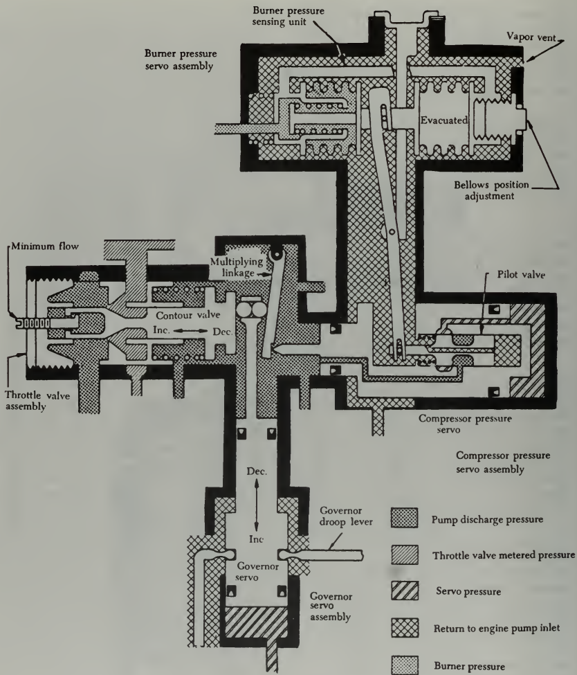
FIGURE 3-50. Computing system.
